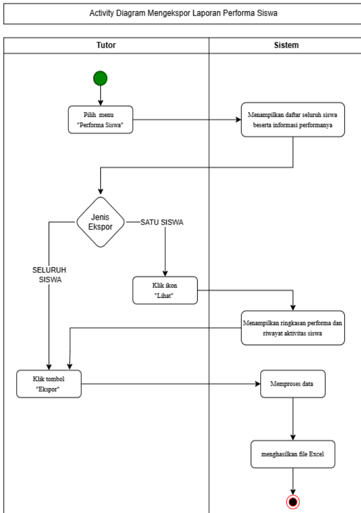
Gambar 6.20 Activity Diagram Tutor Mengekspor Laporan Performa Siswa
