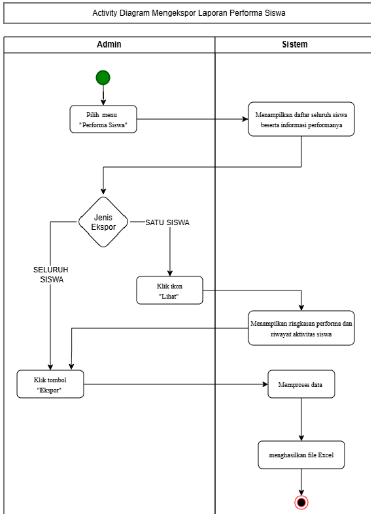
Gambar 6.9 Activity Diagram Mengekspor Laporan Performa Siswa
