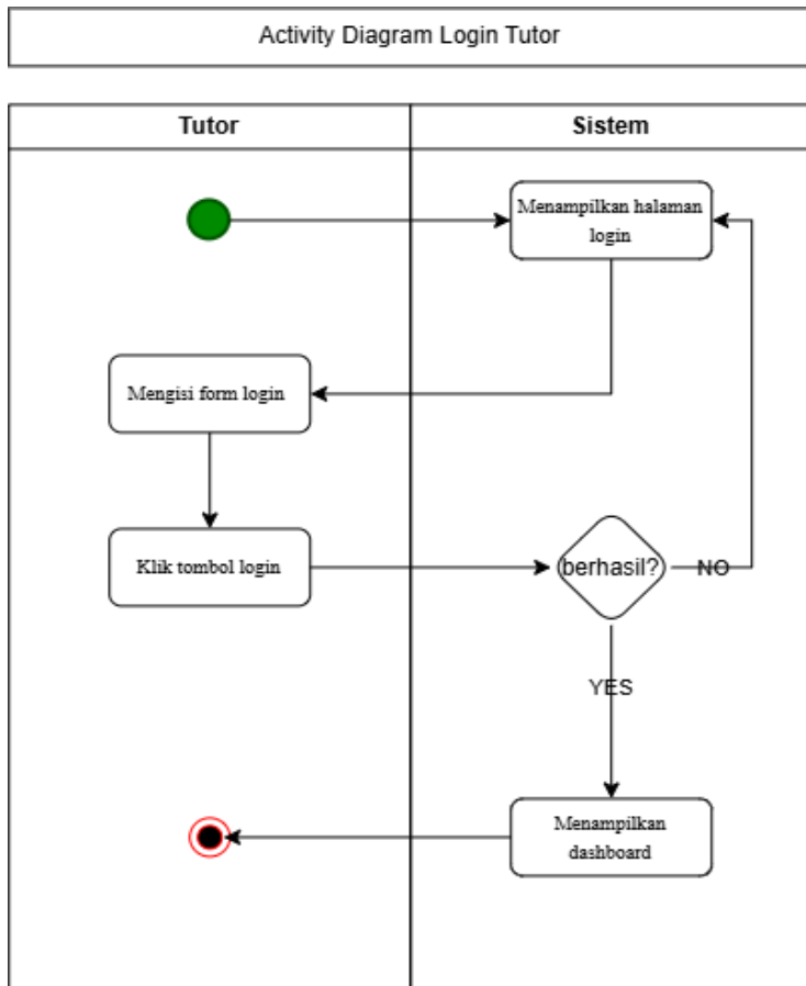
Gambar 6.14 Activity Diagram Login Tutor
