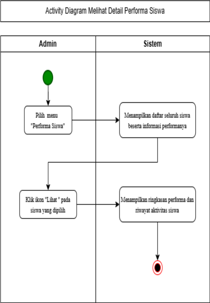
Gambar 6.7 Activity Diagram Melihat Detail Performa Siswa
