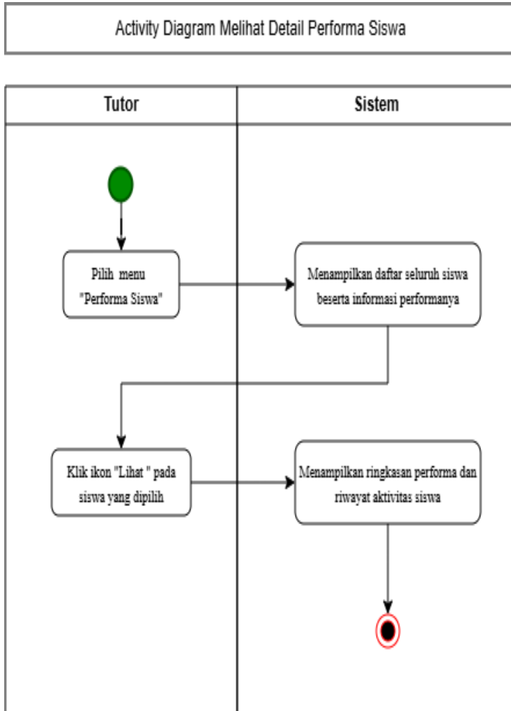
Gambar 6.18 Activity Diagram Tutor Melihat Detail Performa Siswa
