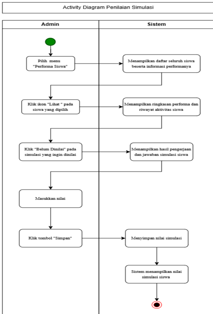
Gambar 6.8 Activity Diagram Penilaian Simulasi
