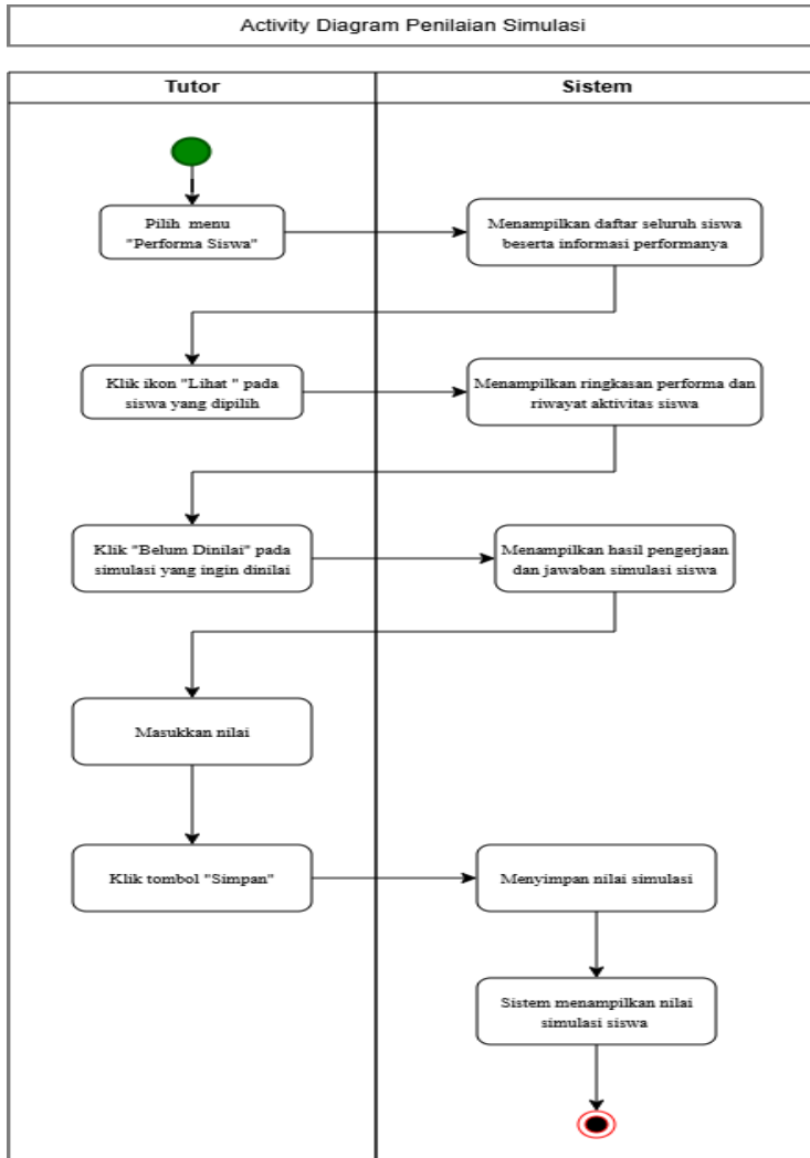
Gambar 6.19 Activity Diagram Tutor Penilaian Simulasi
