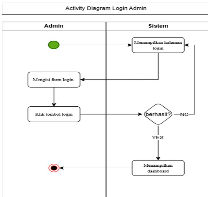
Gambar 6.1 Activity Diagram Login Admin
