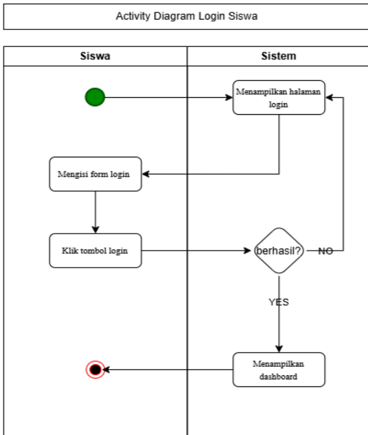
Gambar 6.21 Activity Diagram Login Siswa
