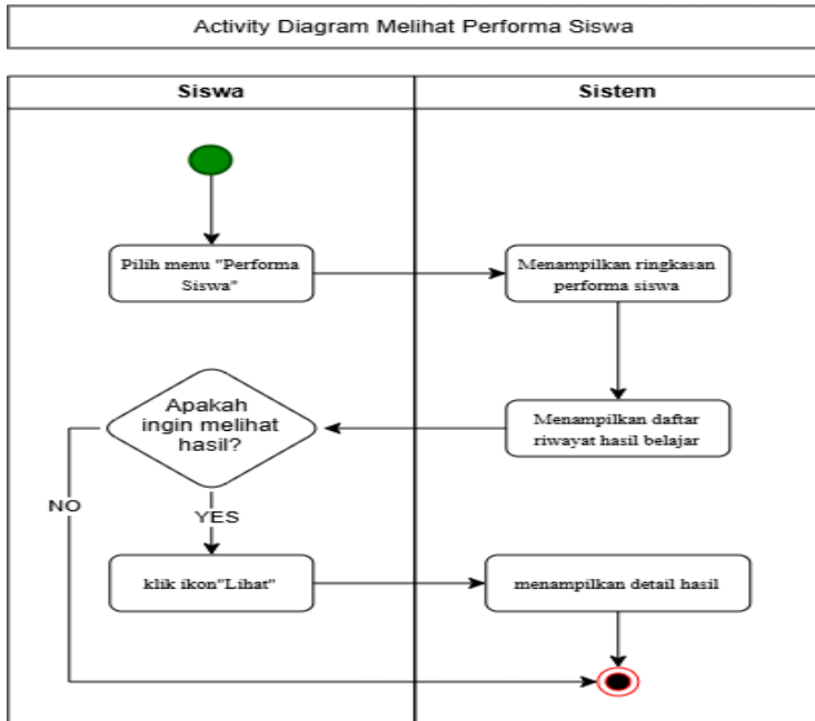
Gambar 6.23 Activity Diagram Siswa Melihat Performa
